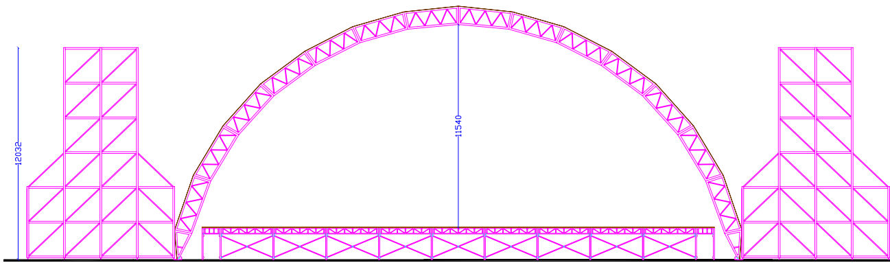
FRONTAL ELEVATION
