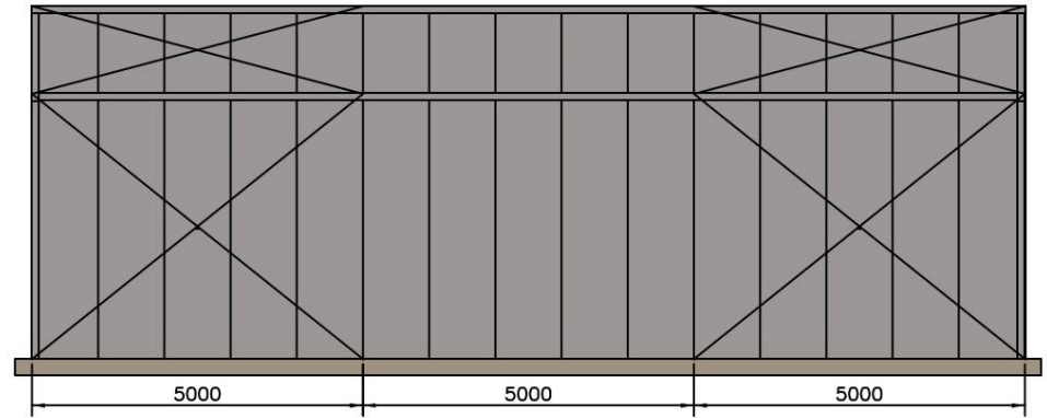
Left Elevation (Scale = 1:125)
