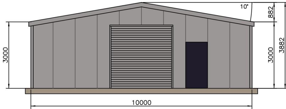
Front Elevation (External)
