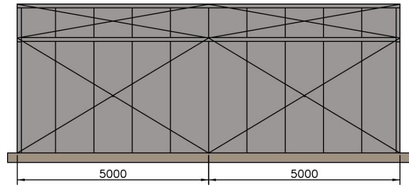
Left Elevation (Scale = 1 :100)
